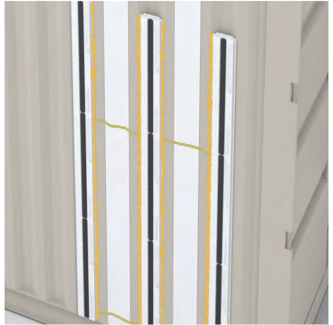
Place PL Premium horizontally and spray foam along the edges.
